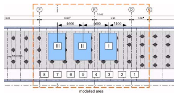
Figure 4: Positions of the mud pumps and alignment of the piles, first design.
